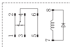
with diode (D type)
