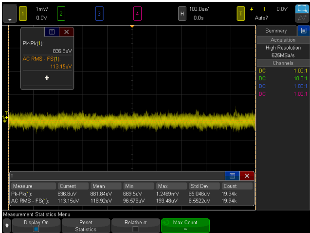
Figure 42. Getting 113 \mu\text{V}_{\text{rms}} noise floor at 1 mV/div with the high resolution mode.
