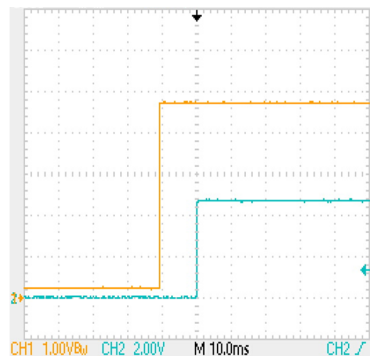
Figure 27. UVP Recovery
