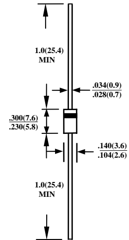
CASE : DO15 DIMENSIONS IN INCHES AND (MILLIMETERS)
