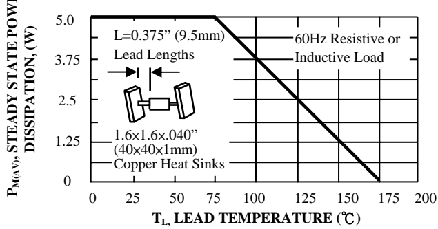
FIG. 5 - STEADY STATE POWER DERATING CURVE
