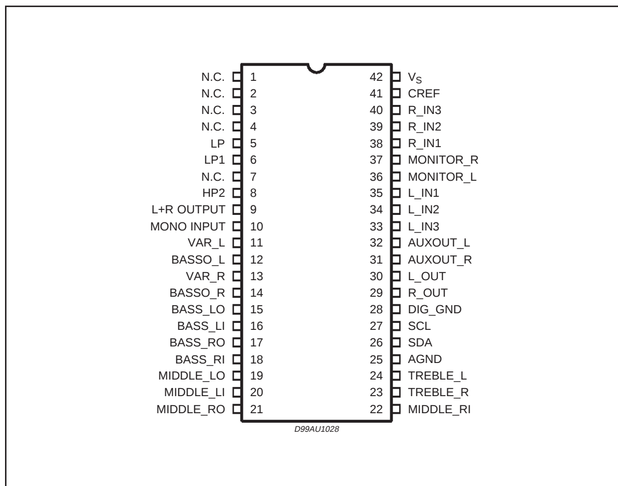
Figure 2. Pin Connection
