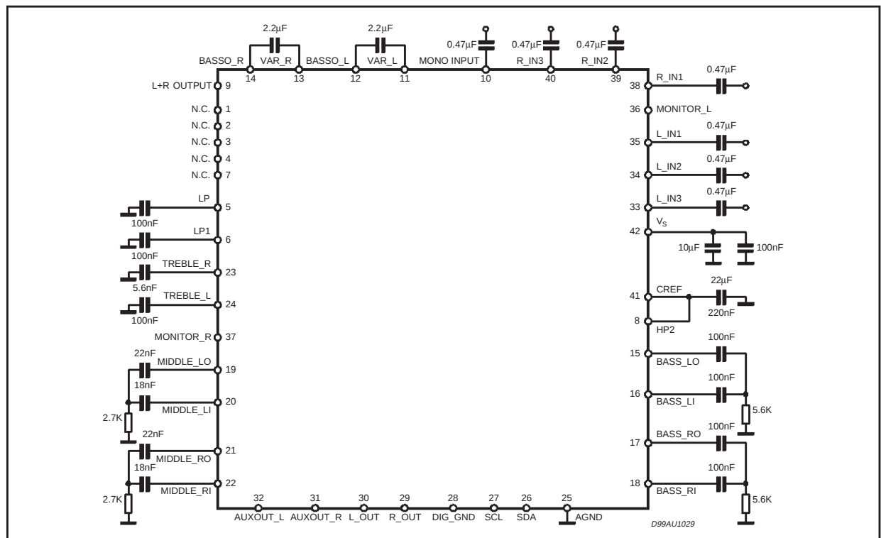
Figure 1. Test Circuit
