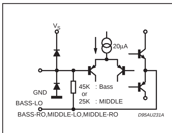
Figure 16. Pin: BASS-LI, BASS-RI, MIDDLE-LI, MIDDLE-R
