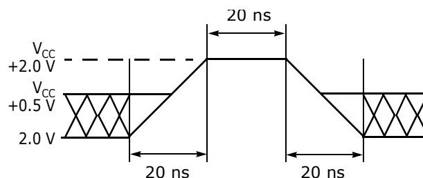
Maximum Positive Overshoot Waveform
