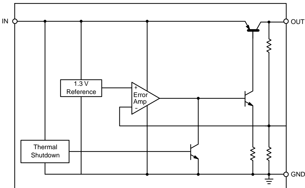
Figure 1. Block Diagram
