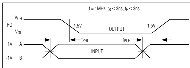
Figure 10. Receiver Propagation Delays
