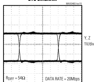
EYE DIAGRAM
