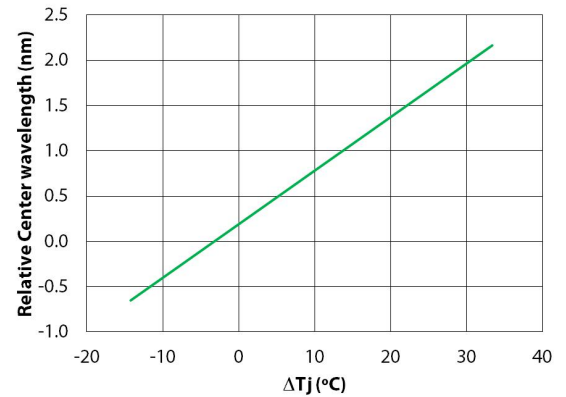
Relative Center Wavelength vs. Temperature
