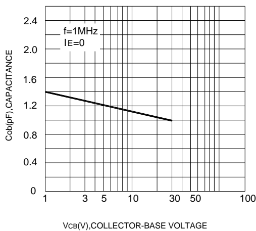
OUTPUT CAPACITANCE
