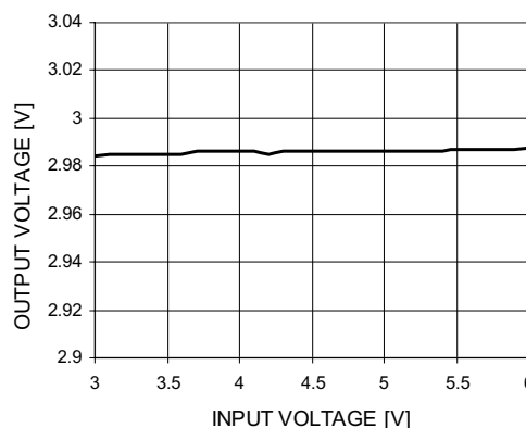
Figure 5. Line Regulation ( I_{LOAD}=5mA )
