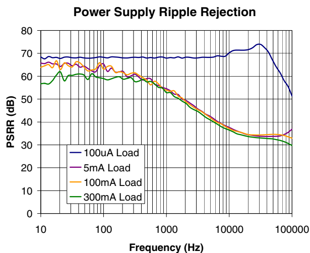
Figure 27. Power Supply Ripple Rejection (No C_{OUT} , C_{BYP}=100nF )
