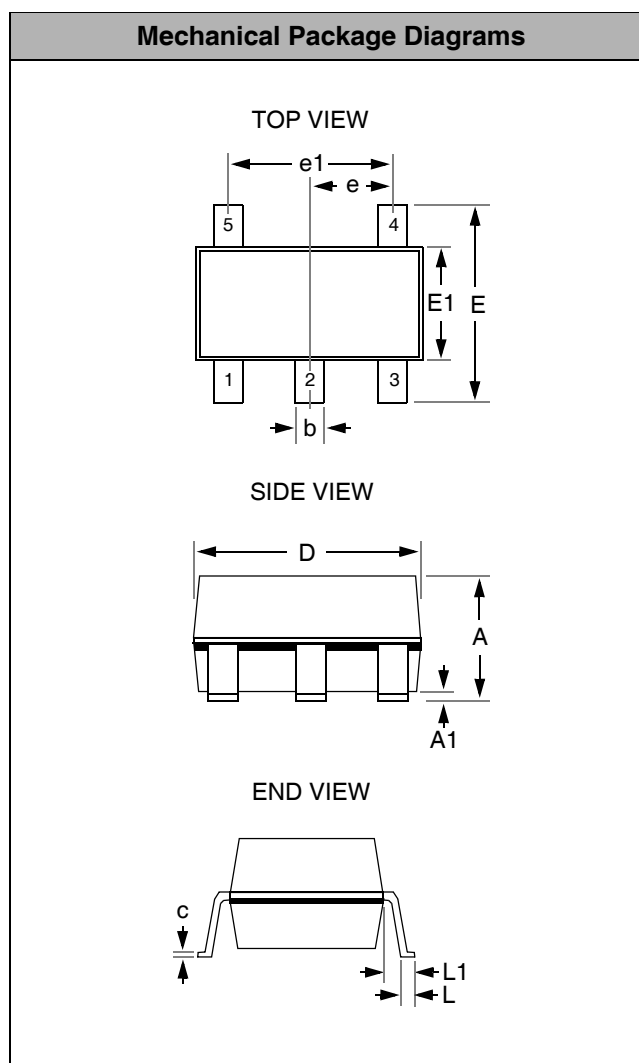
Package Dimensions for SOT23-5.
