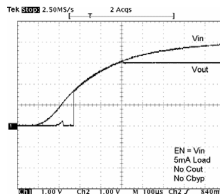
Figure 22. Power-Up ( EN=V_{IN} , I_{LOAD}=5mA , No C_{OUT} , No C_{BYP} )
