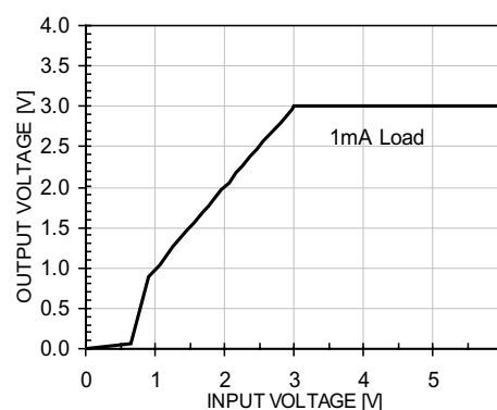
Figure 6. Line Regulation ( I_{LOAD}=1mA )
