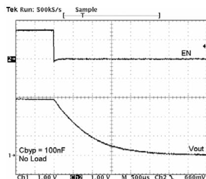
Figure 21. Disable Response ( C_{BYP}=100nF , No Load)
