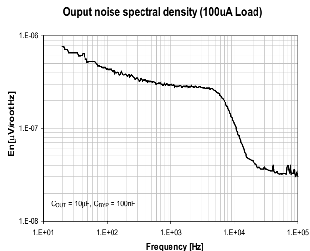
Figure 28. Output Noise Spectral Density ( I_{LOAD}=100\mu A , C_{OUT}=10\mu F , C_{BYP}=100nF )
