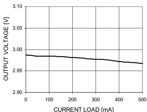
Figure 1. Load Regulation
