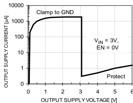
Figure 12. Output Supply Current vs. Voltage
