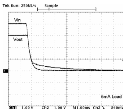
Figure 24. Power-Down ( I_{LOAD}=5mA )
