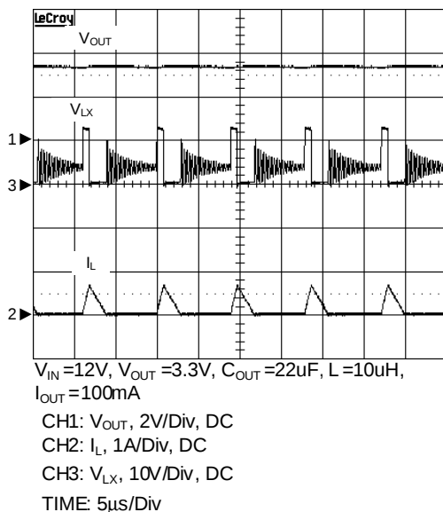
Normal Operation in Light Load
