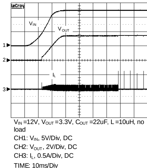
Power On
