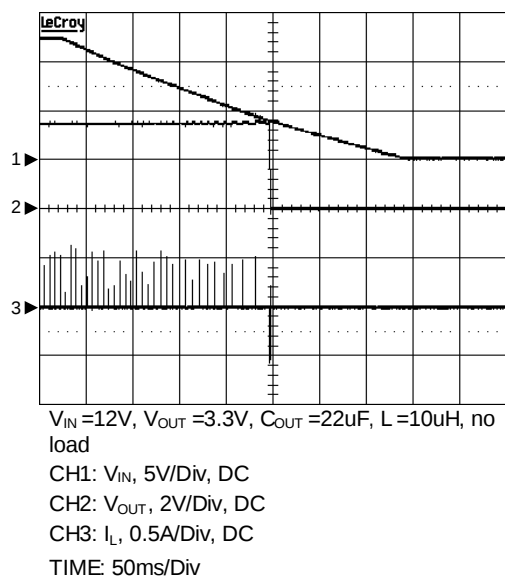
Power Off
