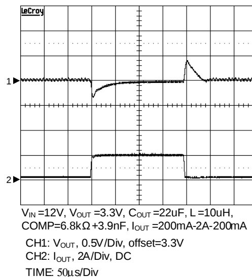
Load Transient
