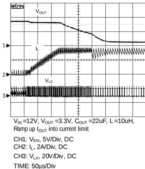
Current Limit & Frequency Foldback
