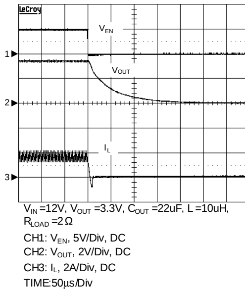
Shutdown
