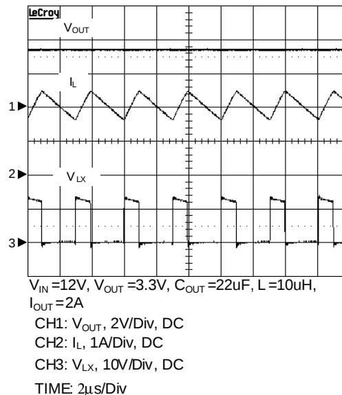
Normal Operation in Heavy Load
