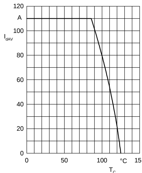
Fig. 2 DC output current at case temperature
