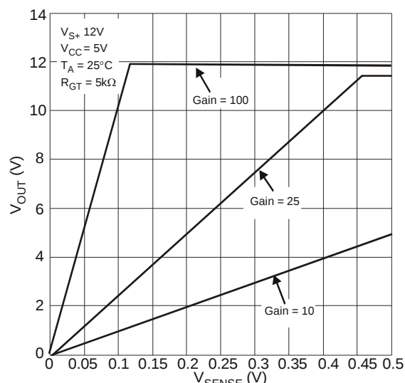
Output Voltage vs. V_{SENSE}
