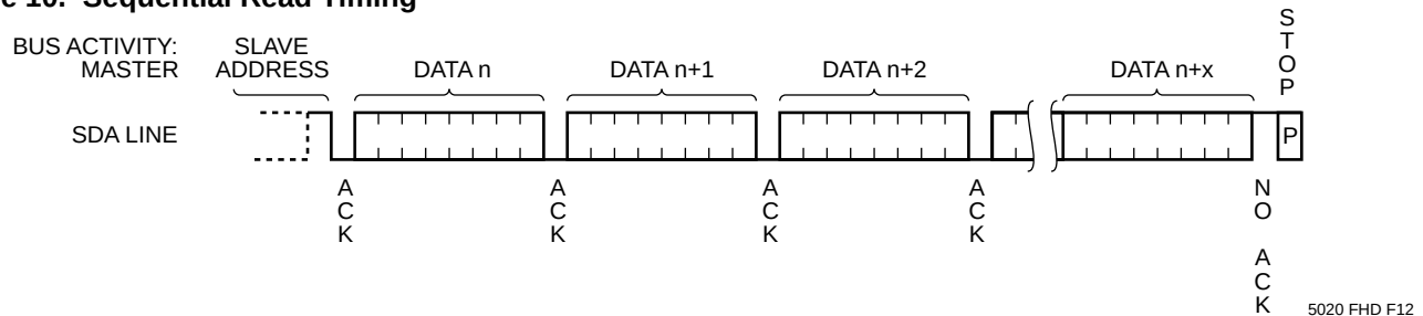
Figure 10. Sequential Read Timing
