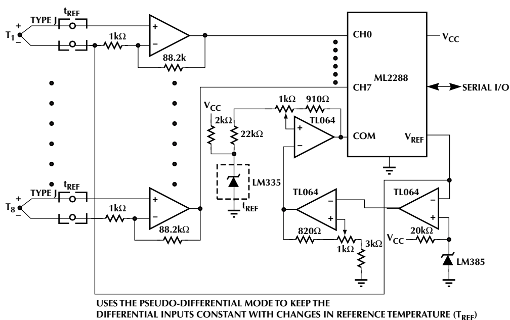
Convert 8 Thermocouples with only One Cold-Junction Compensator
