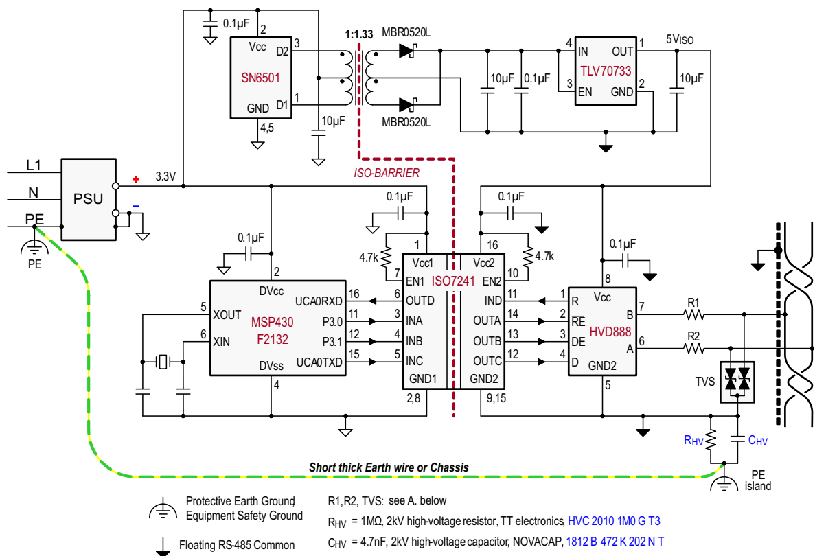
Figure 24. Isolated Bus Node With Transient Protection
