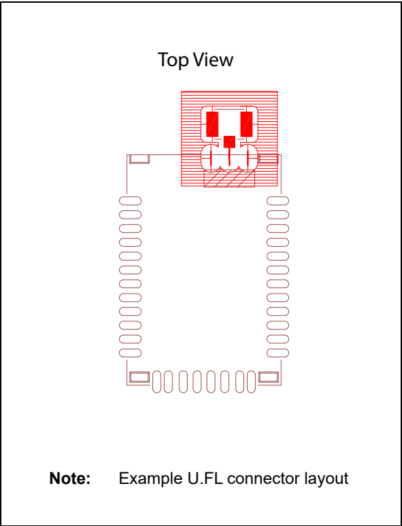
FIGURE 2-4: RN42N MODULE MOUNTING DETAILS
