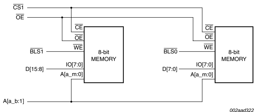
Fig 21. Booting from two 8-bit memory chips
