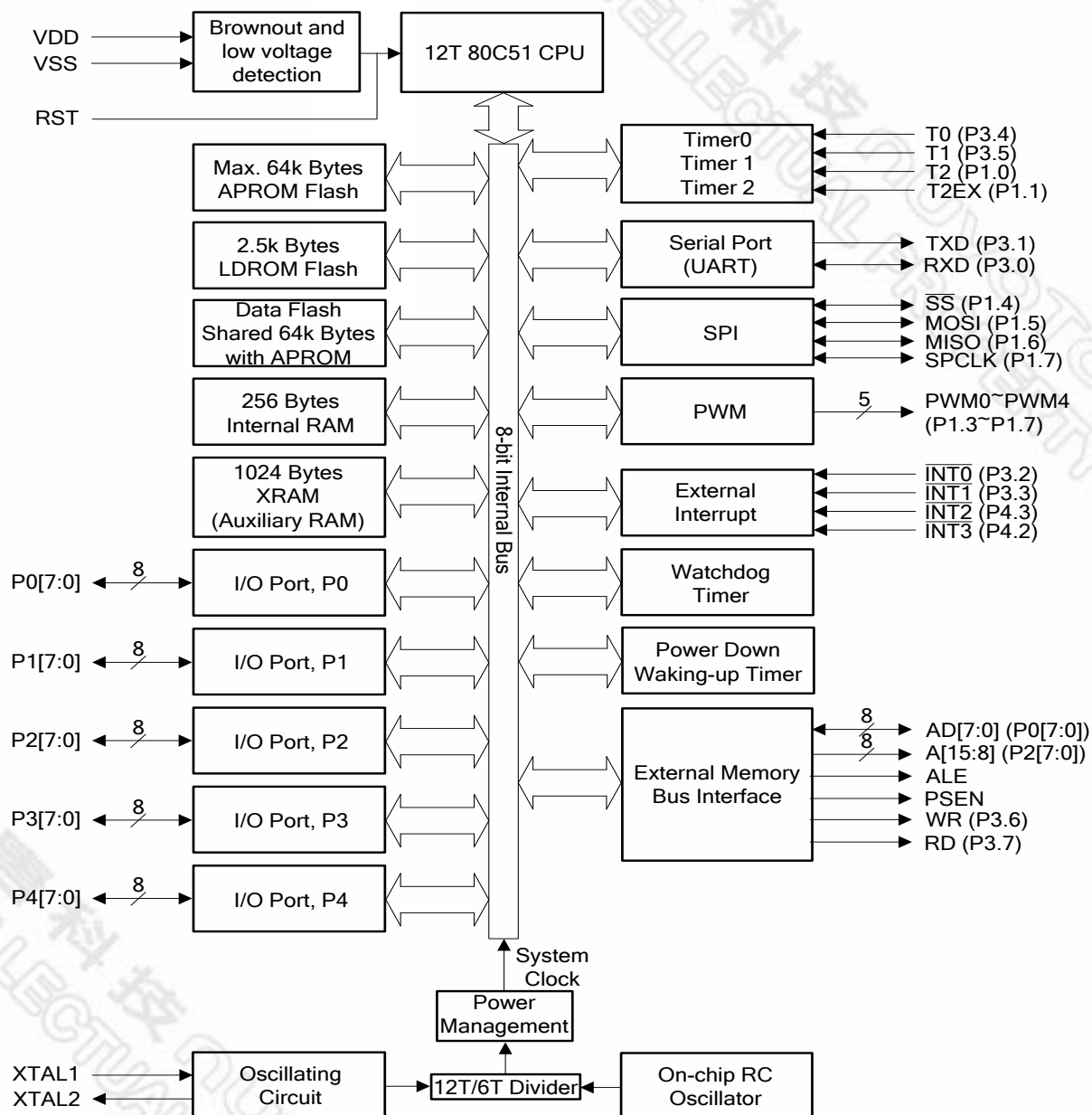
Figure 3–1. N78E517A Function Block Diagram
