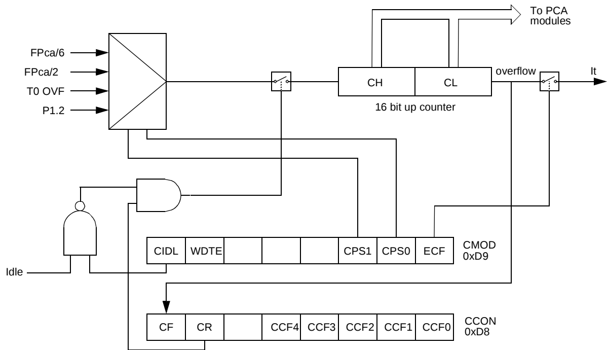
Figure 67. PCA Timer/Counter
