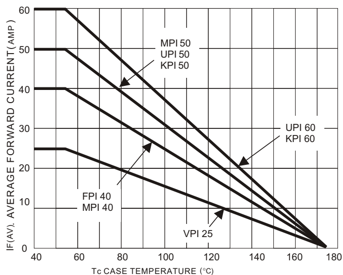
Figure 3 CURRENT DERATING
