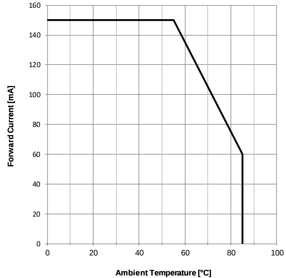
Derating Curve:
