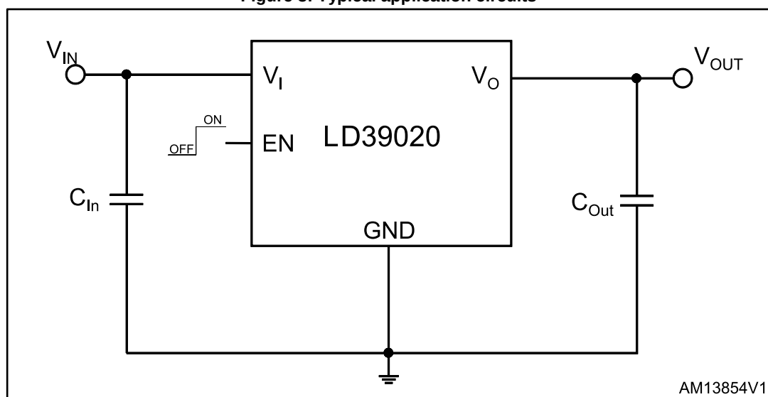
Figure 3: Typical application circuits
