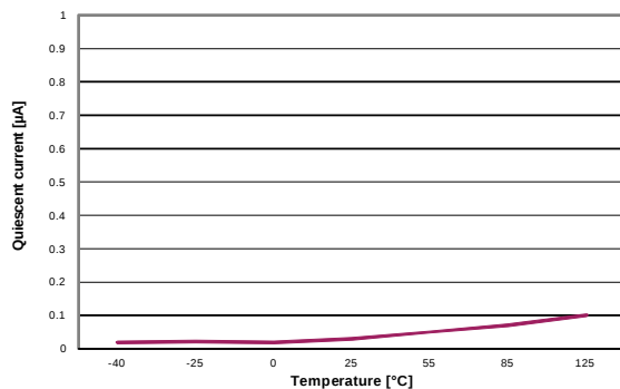
Figure 10: Shutdown current vs. temperature
