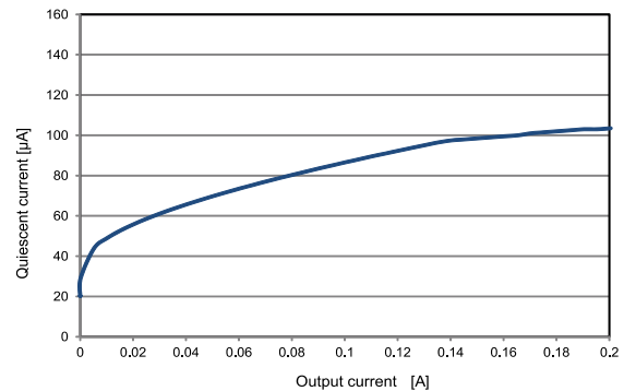
Figure 11: Quiescent current vs. load current
