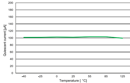
Figure 9: Quiescent current vs. temperature ( I_{OUT} = 200 \text{ mA} )
