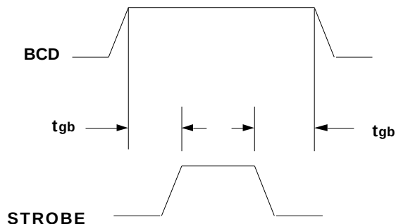
FIGURE 2. GUARD BANDED STROBE
