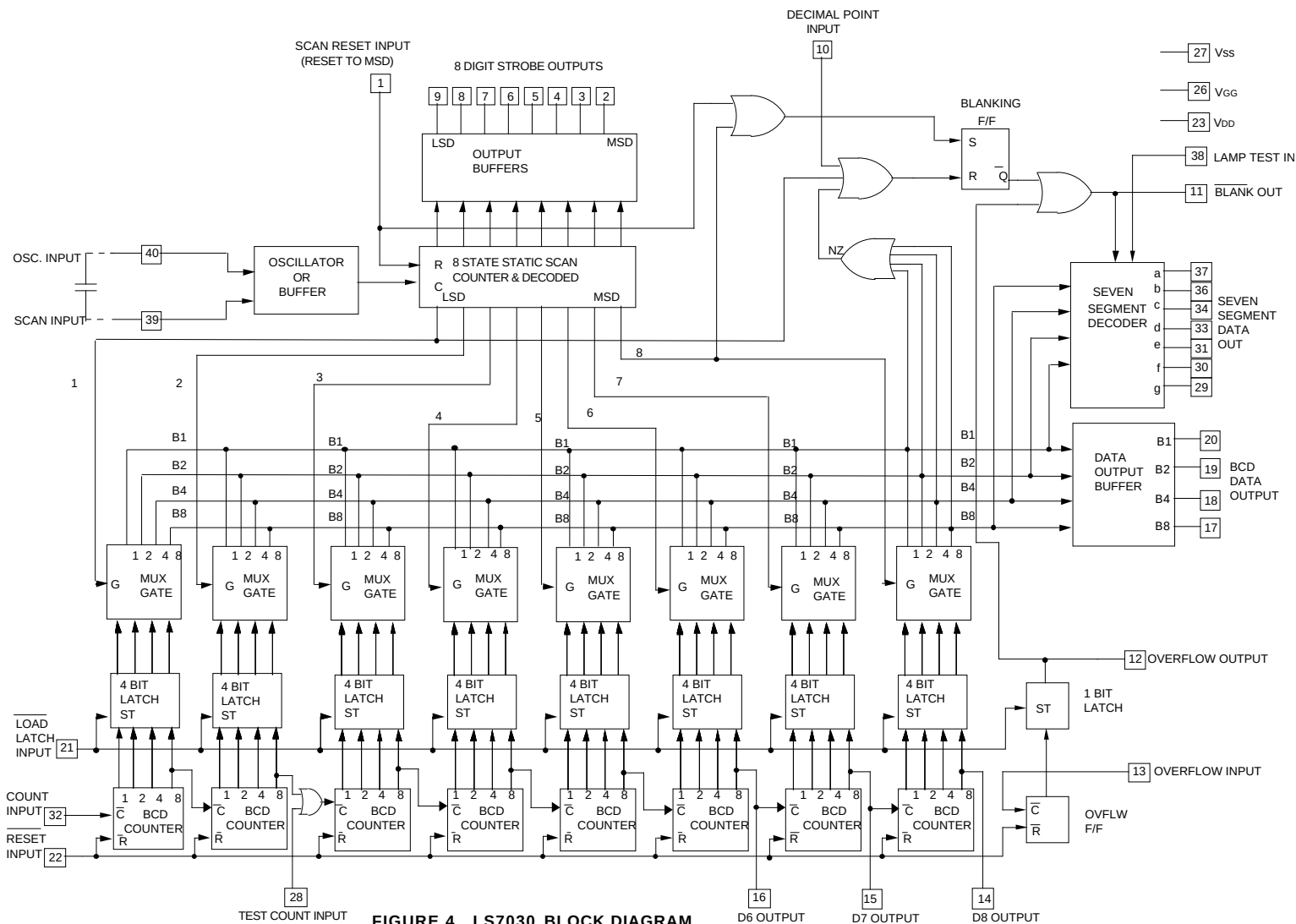
FIGURE 4. LS7030 BLOCK DIAGRAM
