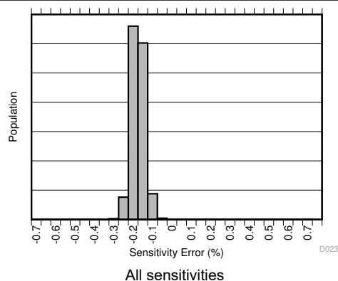
Figure 7-4. Sensitivity Error Production Distribution
