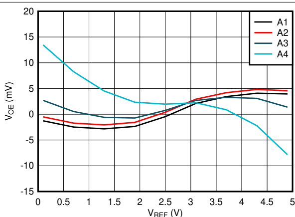
Figure 7-15. Output Voltage Offset vs. V_{REF}
