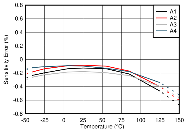
Figure 7-1. Sensitivity Error vs. Temperature
