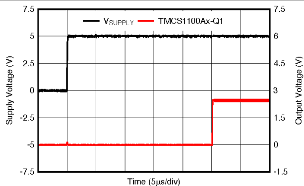
Figure 7-20. Startup Transient Response
