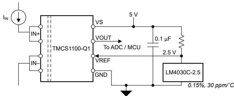
Figure 10-3. TMCS1100-Q1 Example Current-Sense System Design
