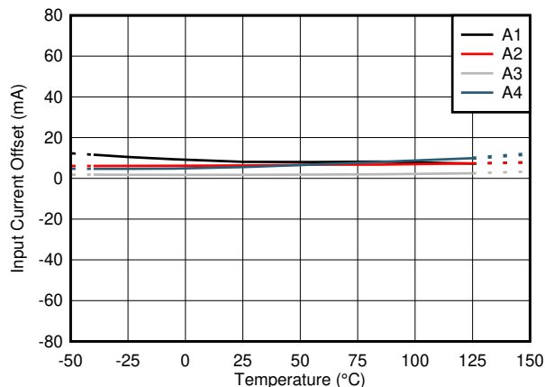
Figure 7-2. Input Offset Current vs. Temperature
