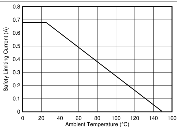
Figure 7-23. Thermal Derating Curve for Safety-Limiting Current, Side 2
