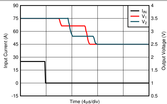
Figure 7-18. Voltage Output Step, Falling
