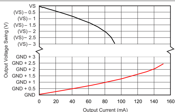
Figure 7-12. Output Swing vs. Output Current
