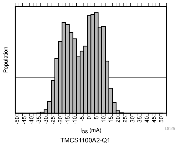
Figure 7-6. Input Offset Current Production Distribution
