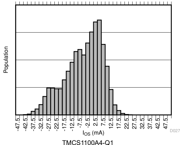
Figure 7-8. Input Offset Current Production Distribution
