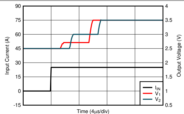
Figure 7-17. Voltage Output Step, Rising
