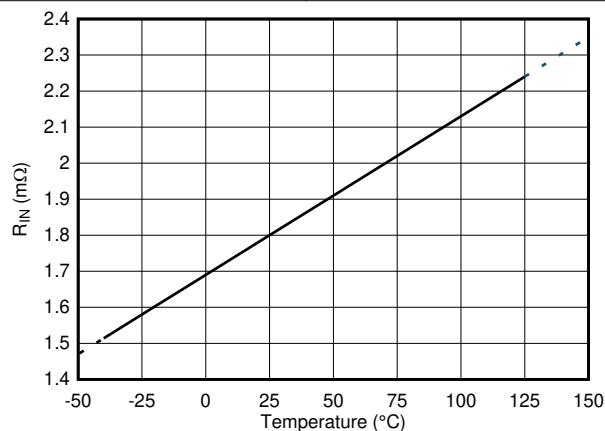
Figure 7-21. Input Conductor Resistance vs. Temperature
