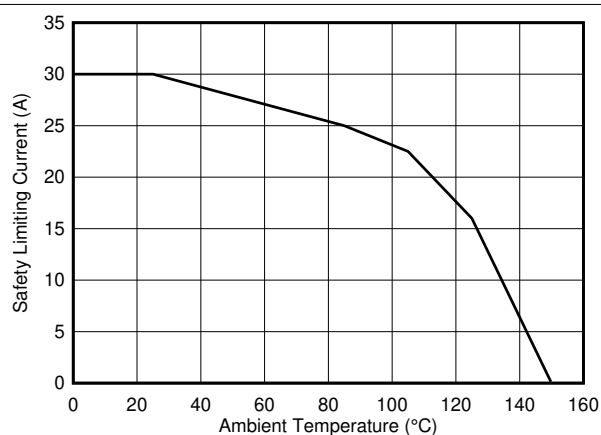
Figure 7-22. Thermal Derating Curve for Safety-Limiting Current, Side 1
