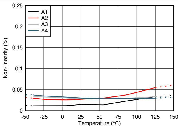
Figure 7-3. Non-Linearity vs. Temperature
