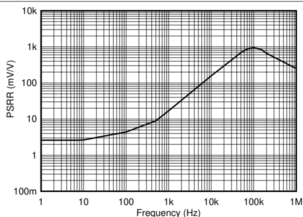
Figure 7-11. PSRR vs. Frequency
