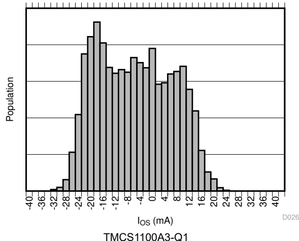
Figure 7-7. Input Offset Current Production Distribution
