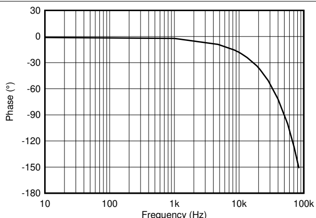
Figure 7-10. Phase vs. Frequency, All Gains
