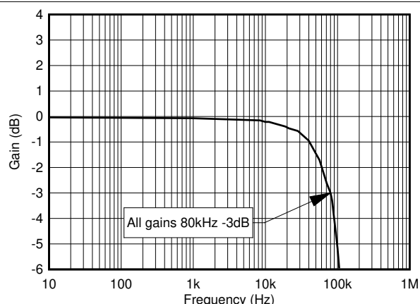
Figure 7-9. Sensitivity vs. Frequency, All Gains Normalized to 1 Hz
