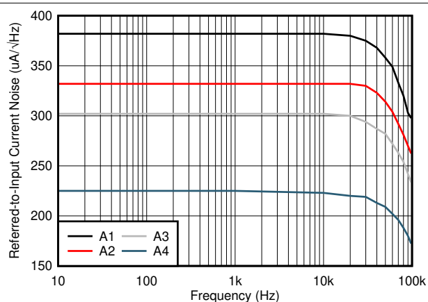
Figure 7-16. Input-Referred Noise vs. Frequency
