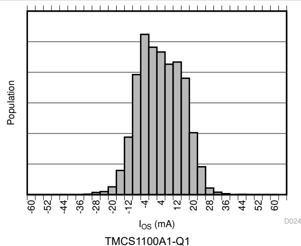
Figure 7-5. Input Offset Current Production Distribution
