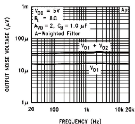
Noise Floor
