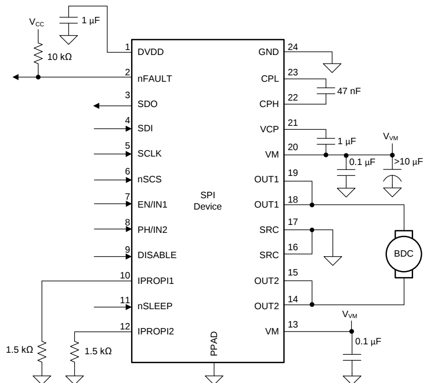
Figure 36. Typical Application Schematic
