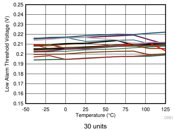
图 7-47. ADC1 Absolute Low Alarm Threshold vs Temperature
