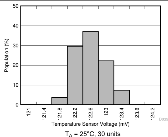
图 7-43. Temperature Sensor Voltage Distribution
