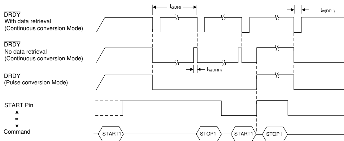
图 9-42. \overline{\text{DRDY}} Operation
