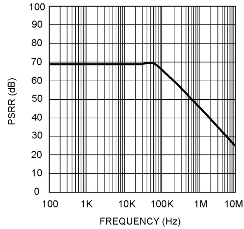
PSRR vs. Frequency @ 5V
