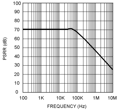
PSRR vs. Frequency @ 12V
