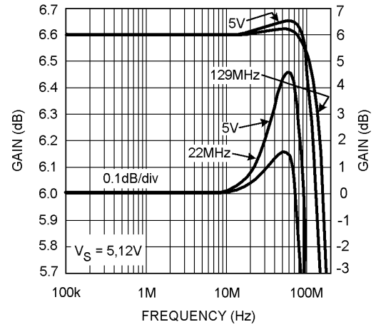
Frequency Response
