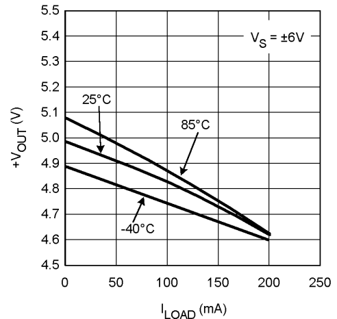
+ V_{OUT} vs. I_{LOAD}
