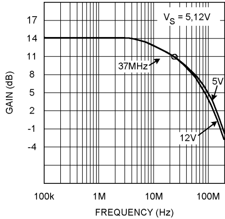
Frequency Response, A_{VCL} = +5\text{V}
