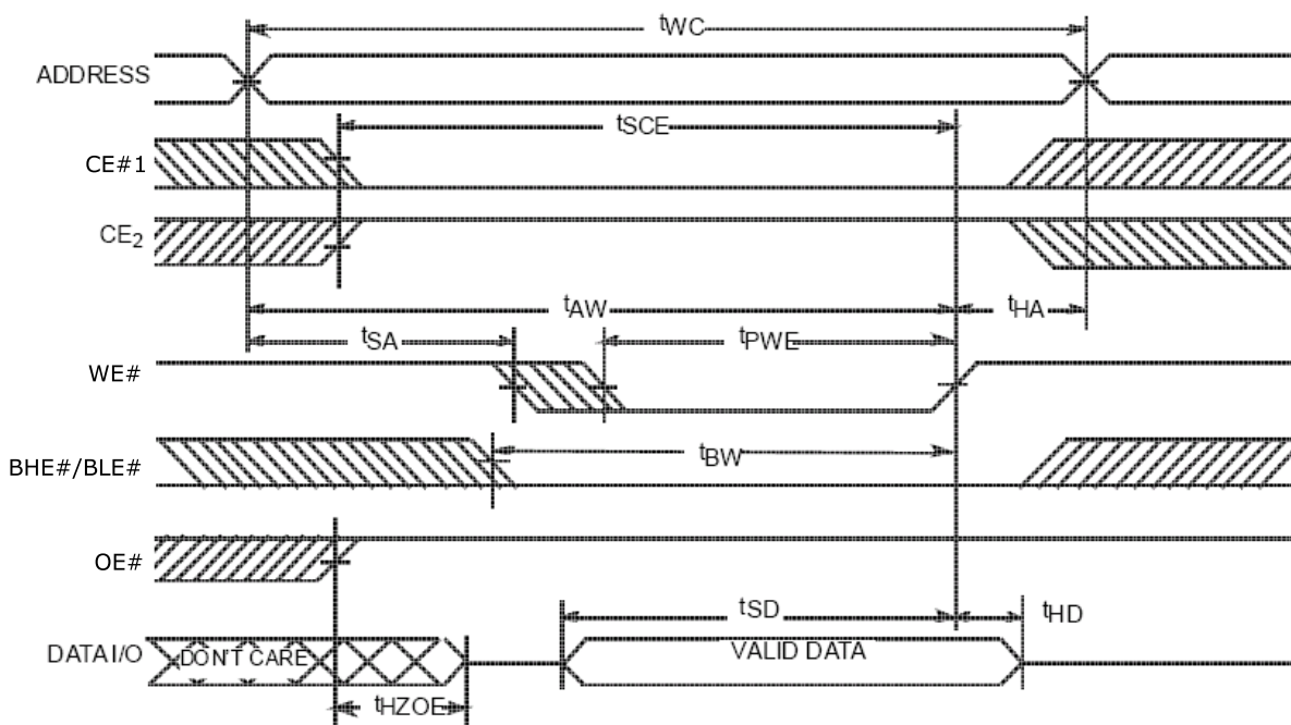
Figure 28. Write Cycle I (WE# Controlled)
