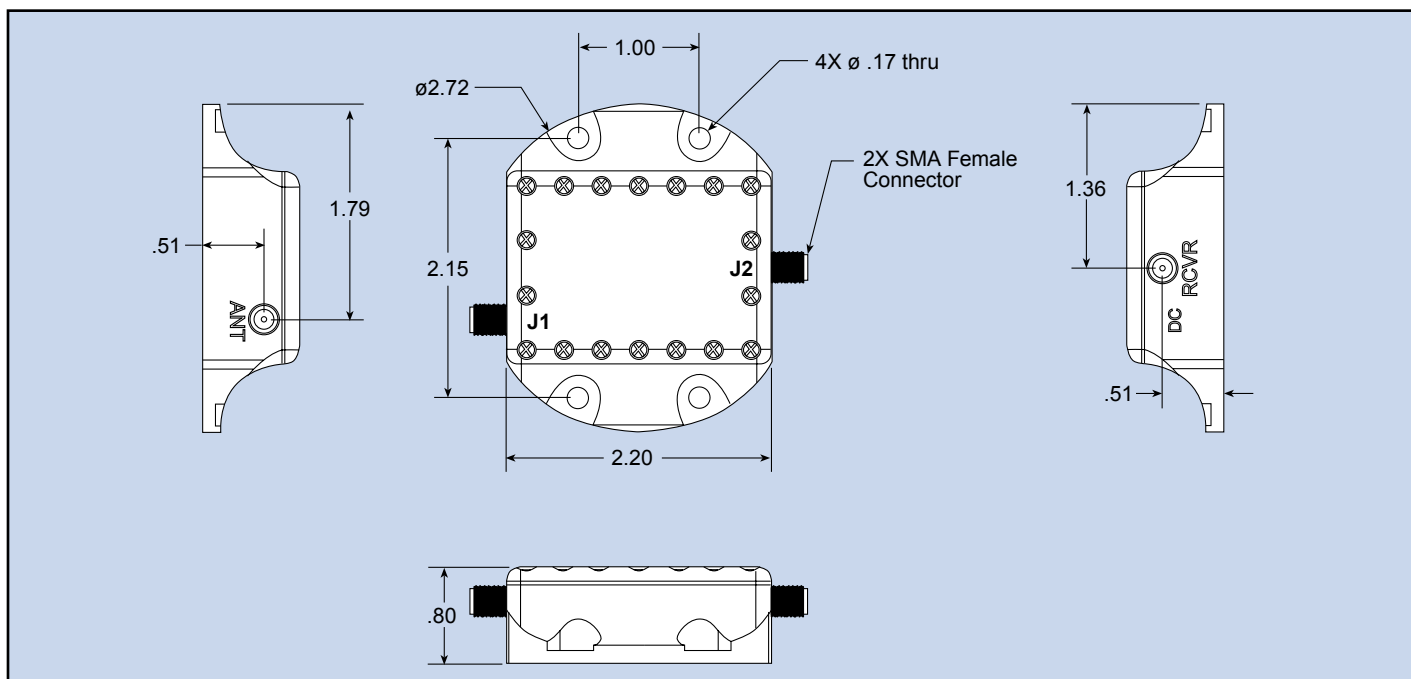
Dimensions (inches)
