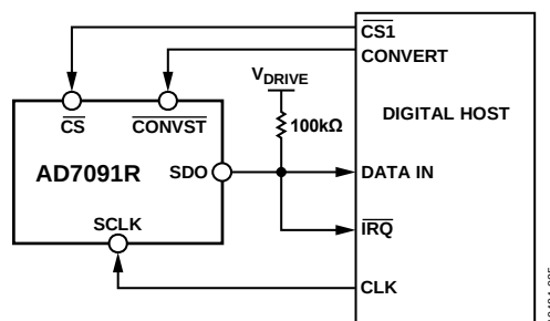
Figure 26. Connection Diagram with BUSY Indicator
