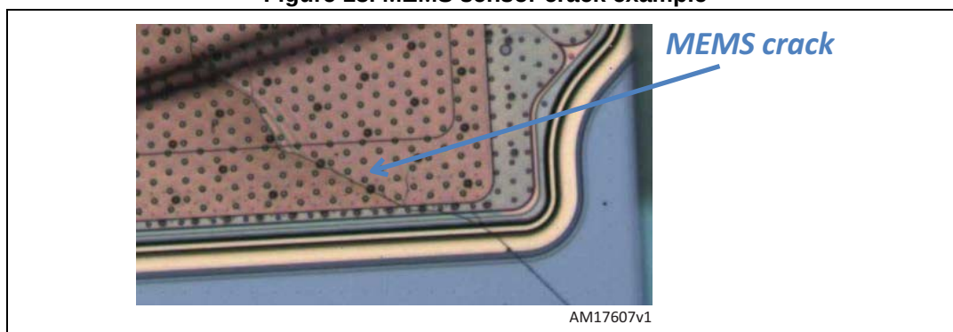
Figure 13. MEMS sensor crack example
