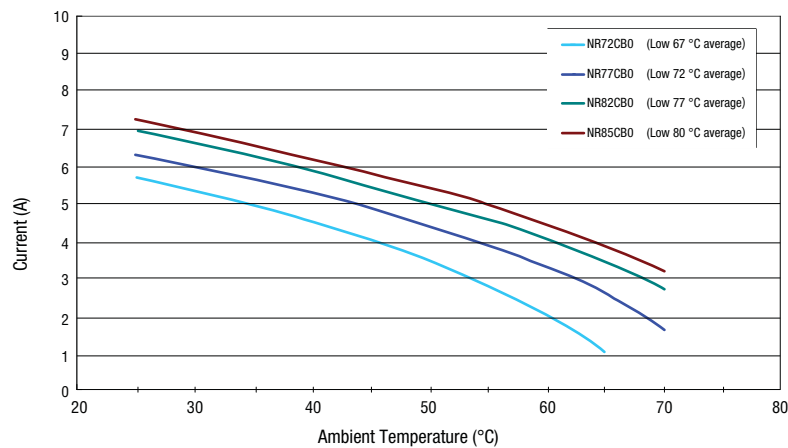
Current vs. Temperature Curves
