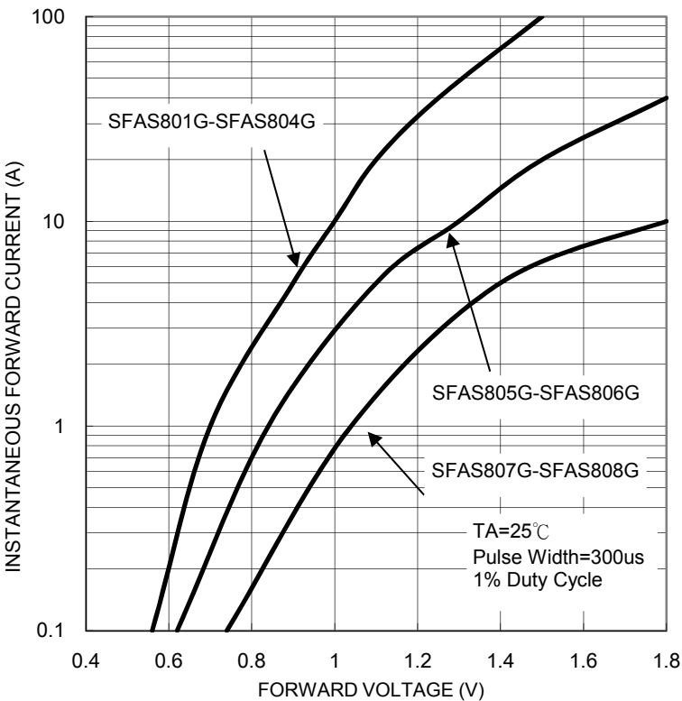
FIG. 5 TYPICAL FORWARD CHARACTERISTICS
