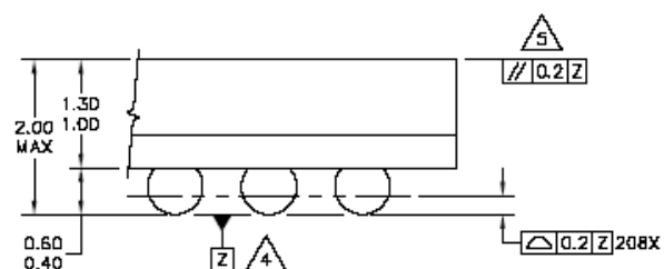
DETAIL K (ROTATED 90° CLOCKWISE)
