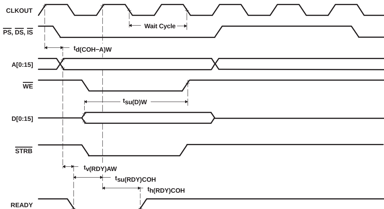
Figure 43. Ready-on-Write Timings
