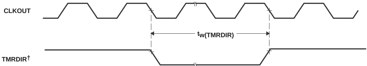
Figure 30. TMRDIR Timing
