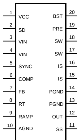
20-Pin HTSSOP Package Top View
