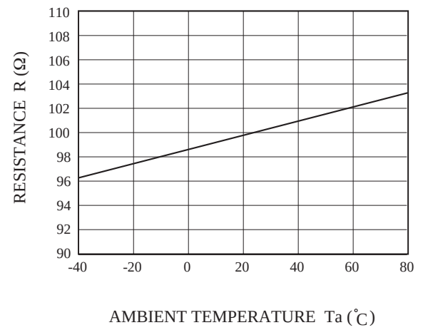
R_{Line} - TEMPERATURE
