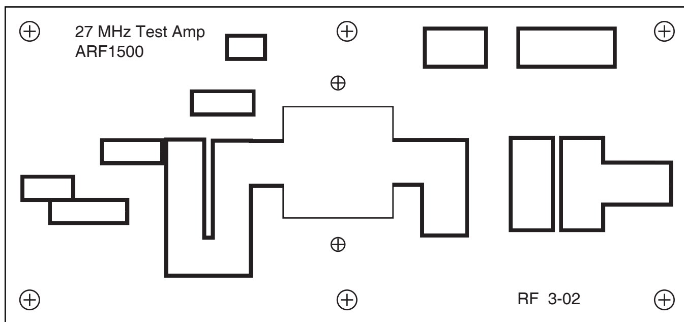
1:1 pcb artwork
