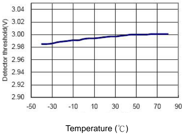
Detector threshold=3.0V
