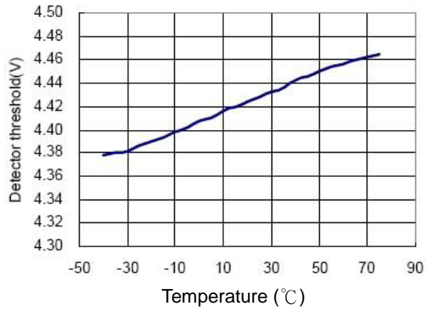
Detector threshold=4.4V
