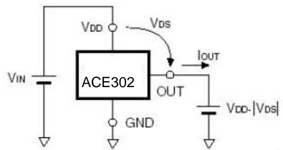
(4) P-ch Drive Output Current Test Circuit
