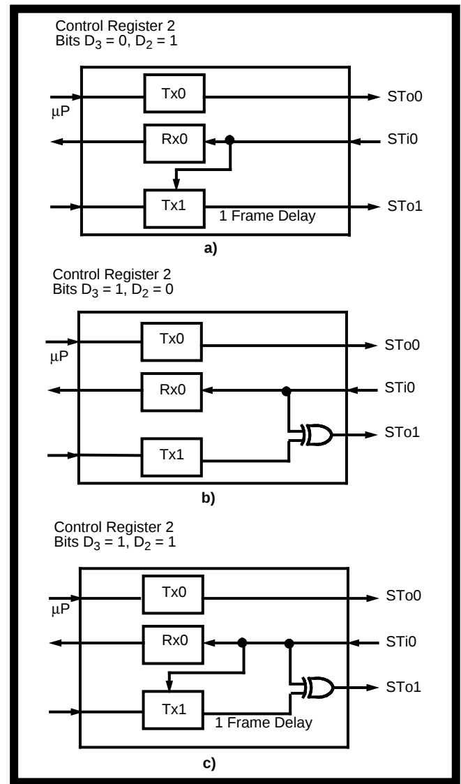
Figure 6 - STo1 Configurations
