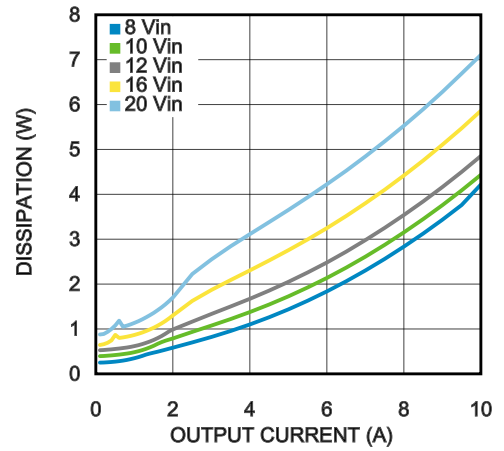
Dissipation 5.0V output @ 25^\circ C
