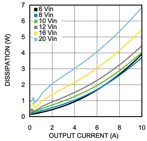
Dissipation 1.8V output @ 25°C
