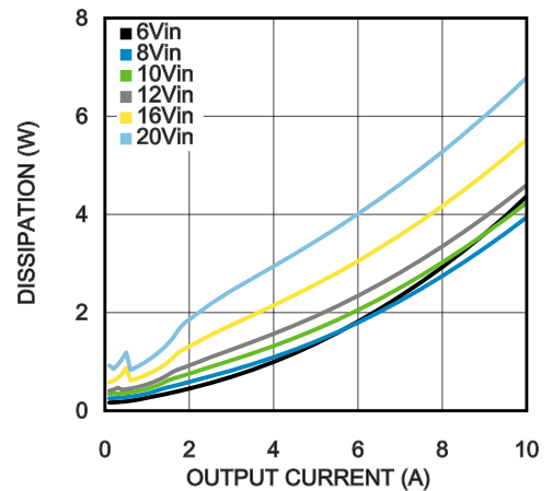
Dissipation 3.3V output @ 25^\circ C
