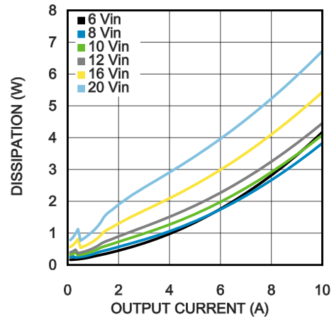
Dissipation 2.5V output @ 25°C
