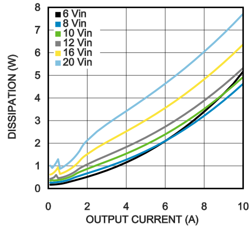
Dissipation 3.3V output @ 85°C
