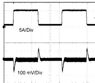
Transient response 12V_{IN} , 3.3V_{OUT} 1 to 10A Step
