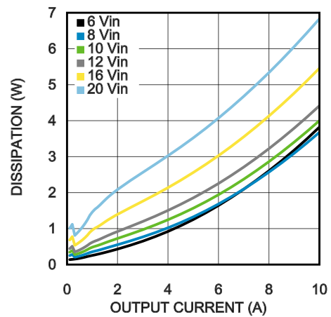
Dissipation 1.5V output @ 25°C
