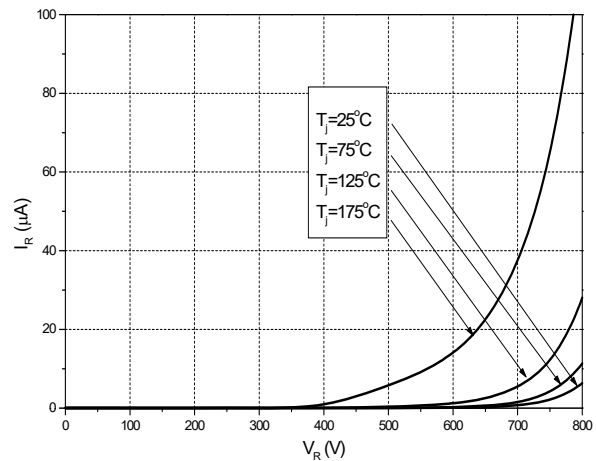
Figure 2. Reverse Characteristics
