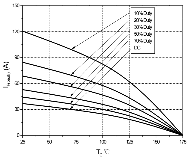
Figure 7. Current Derating
