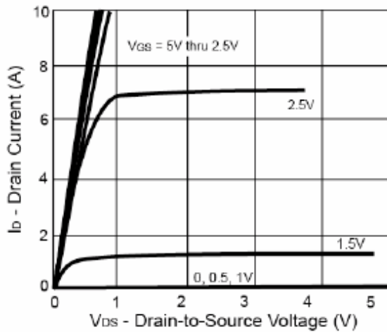
Fig. 1 On-State Characteristics
