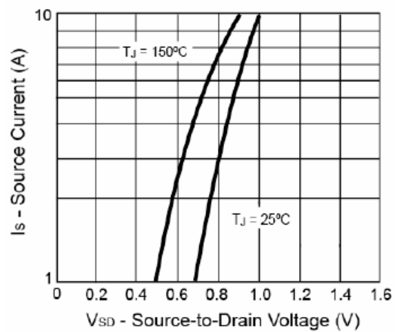
Fig. 4 Diode Forward Voltage vs. Current
