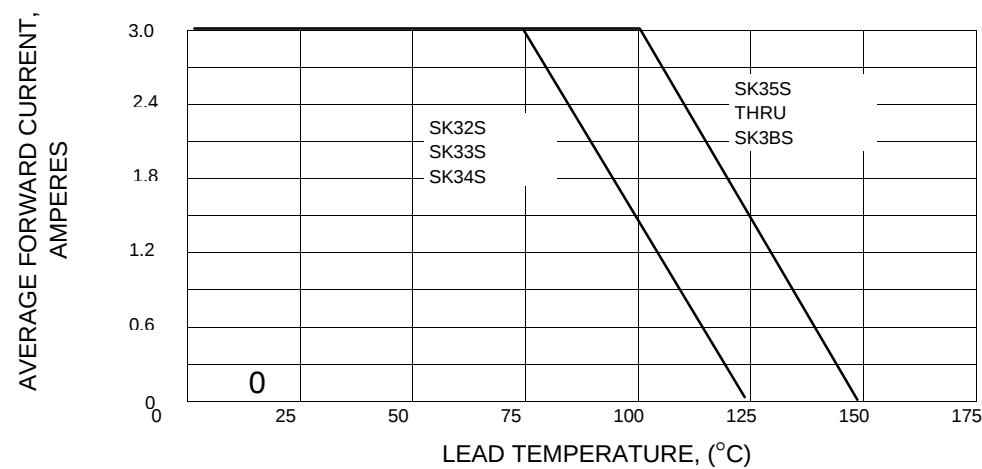
FIG.1 - FORWARD CURRENT DERATING CURVE
