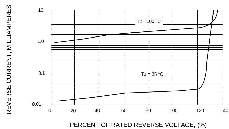
FIG.4 - TYPICAL REVERSE CHARACTERISTICS
