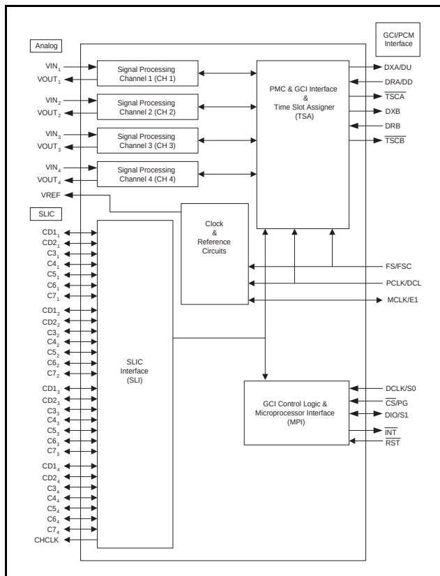
Figure 1 - Block Diagram
