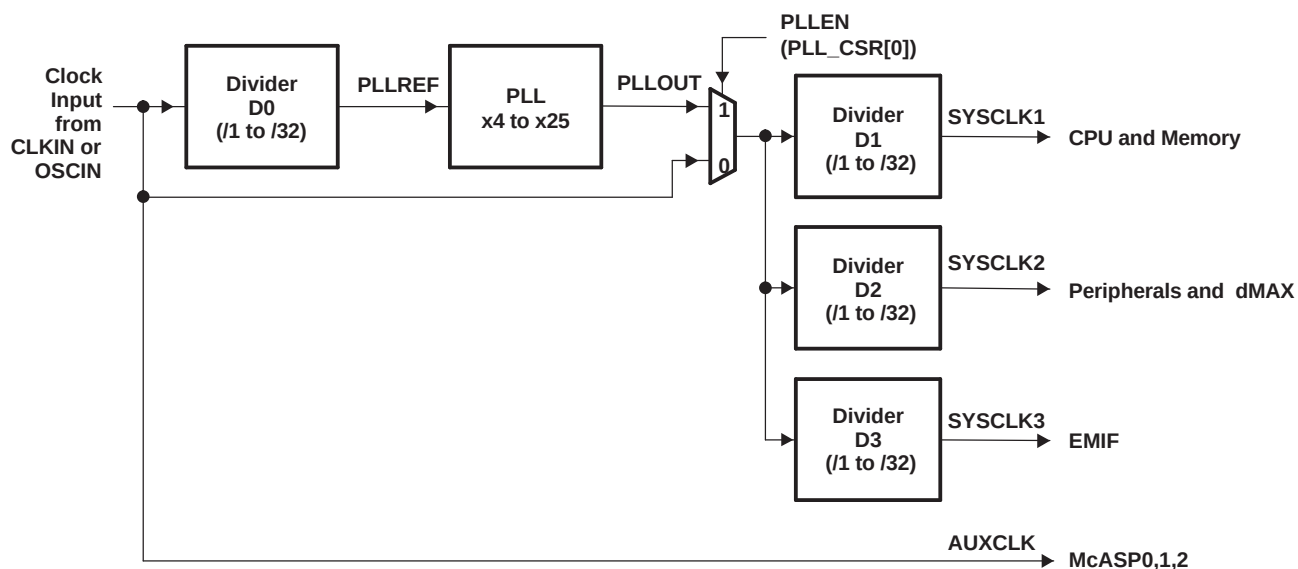
Figure 4-43. PLL Topology
