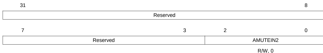
Figure 4-28. CFGMCASP2 Register Bit Layout (0x4000 0020)
