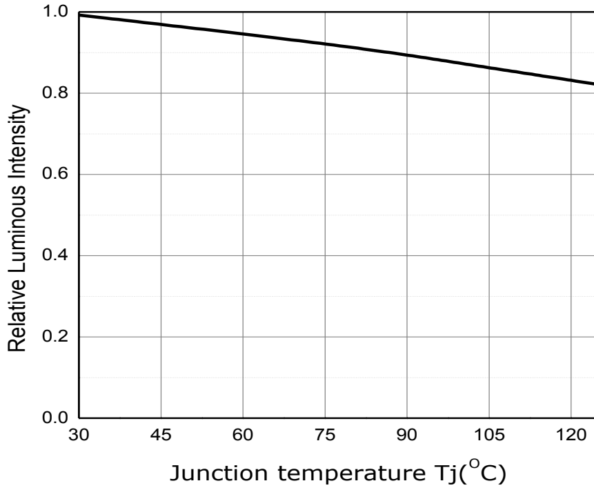
Fig 6. Junction Temperature vs. Relative Luminous Intensity, I_F=100mA
