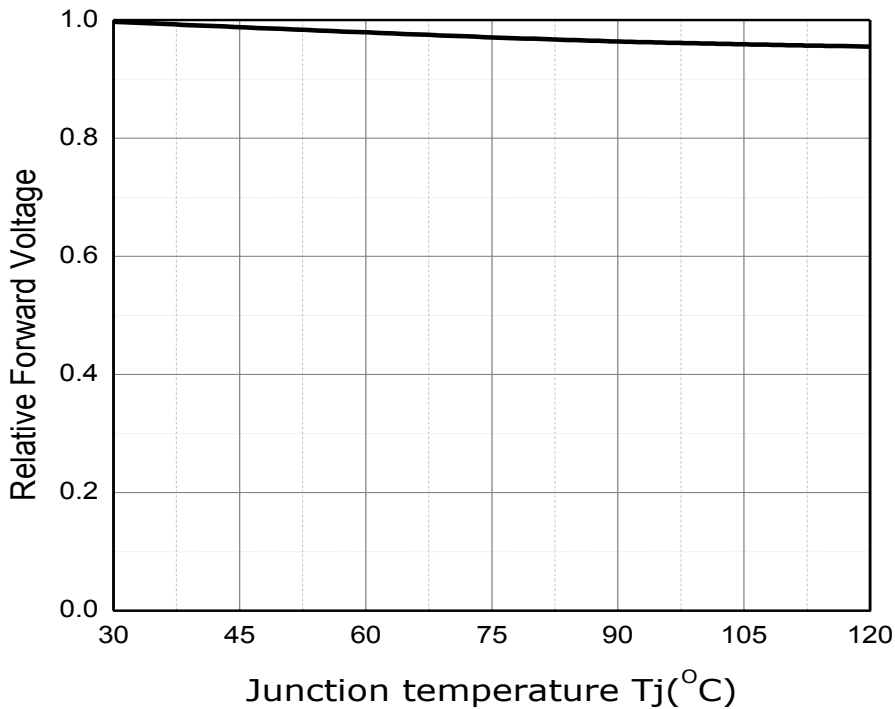
Fig 7. Junction Temperature vs. Relative Forward Voltage, I_F=100mA
